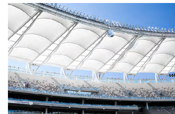
FIBERGLASS MEMBRANES
